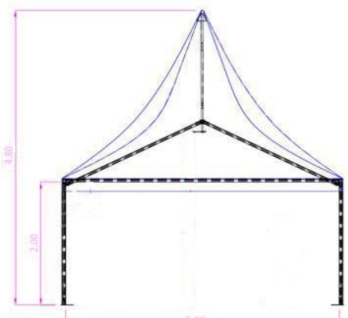
Chapiteau 5x5
